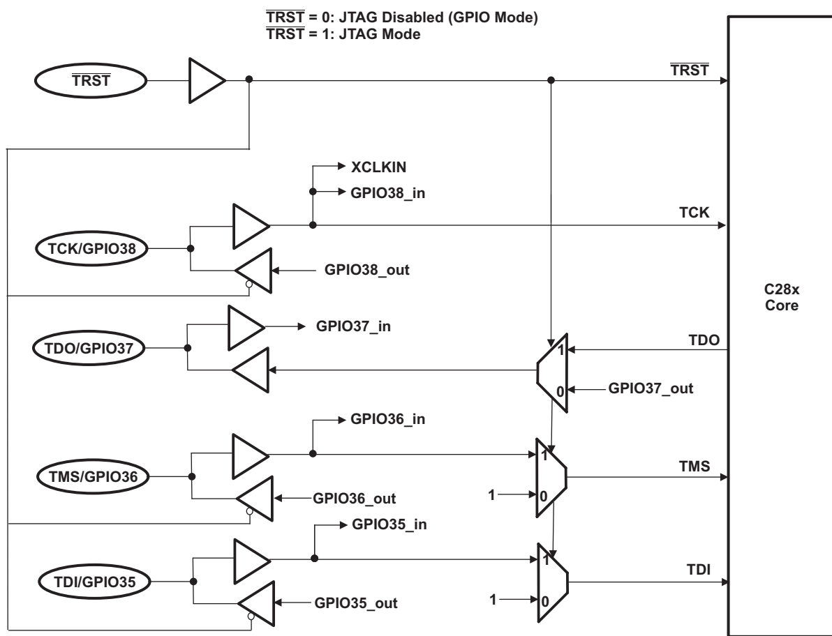
Figure 6-39. JTAG/GPIO Multiplexing
